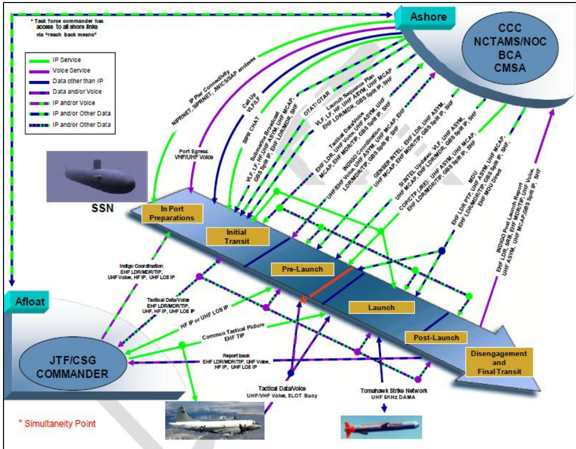
Figure 11. Land Attack/Strike Mission Scenario (from PMW770 2011b, 52)
